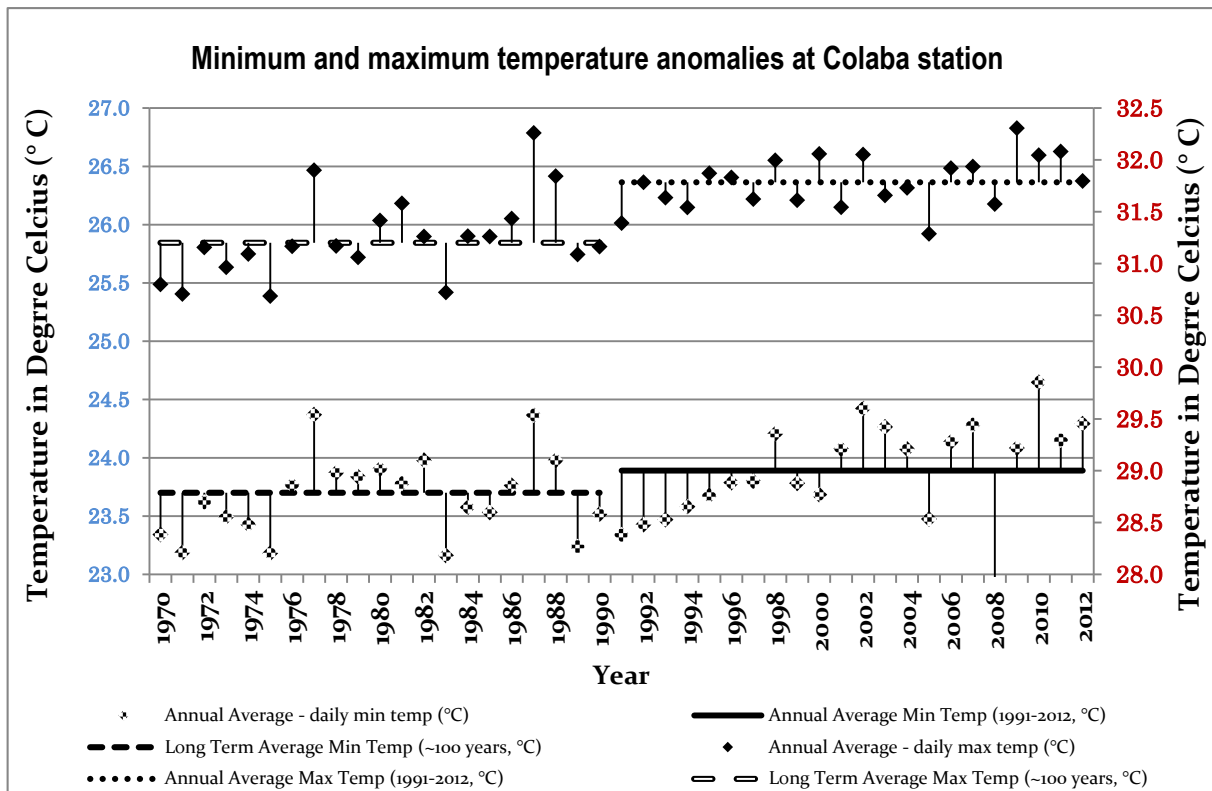
Figure No. 4-13: Minimum and maximum temperature anomalies at Colaba station
