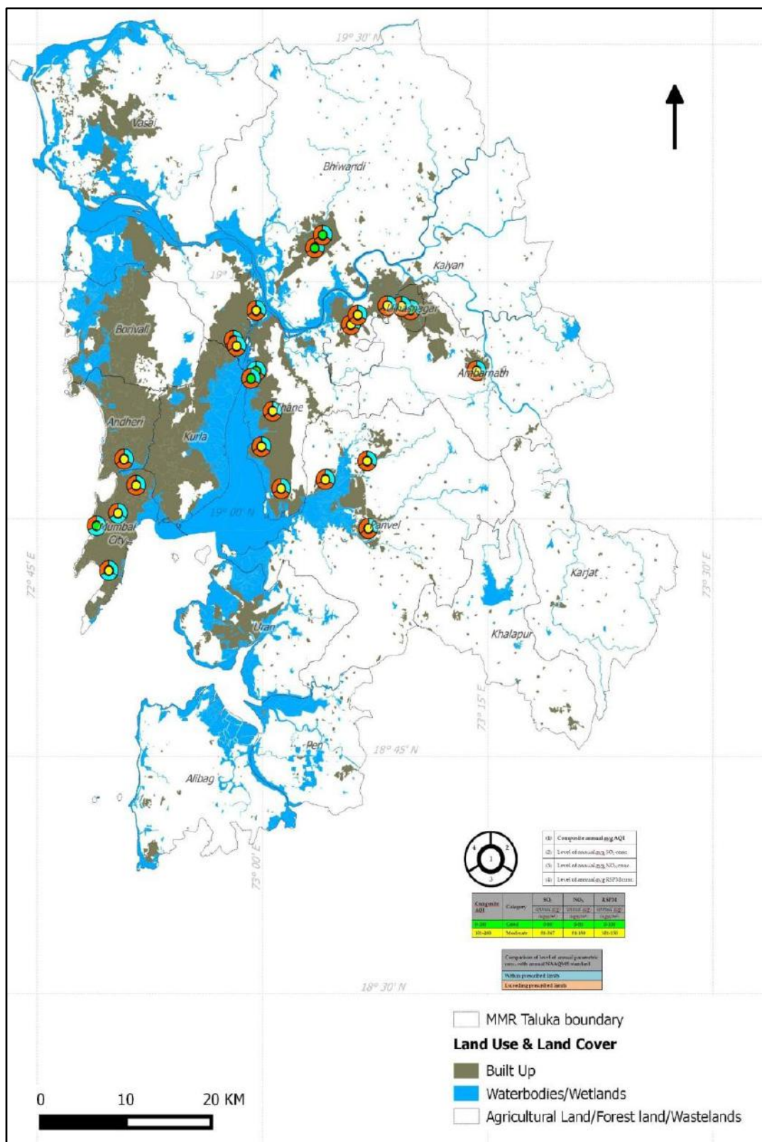
Map No. 3-7: Annual average Air Quality across monitoring locations in Maharashtra 2012-13
